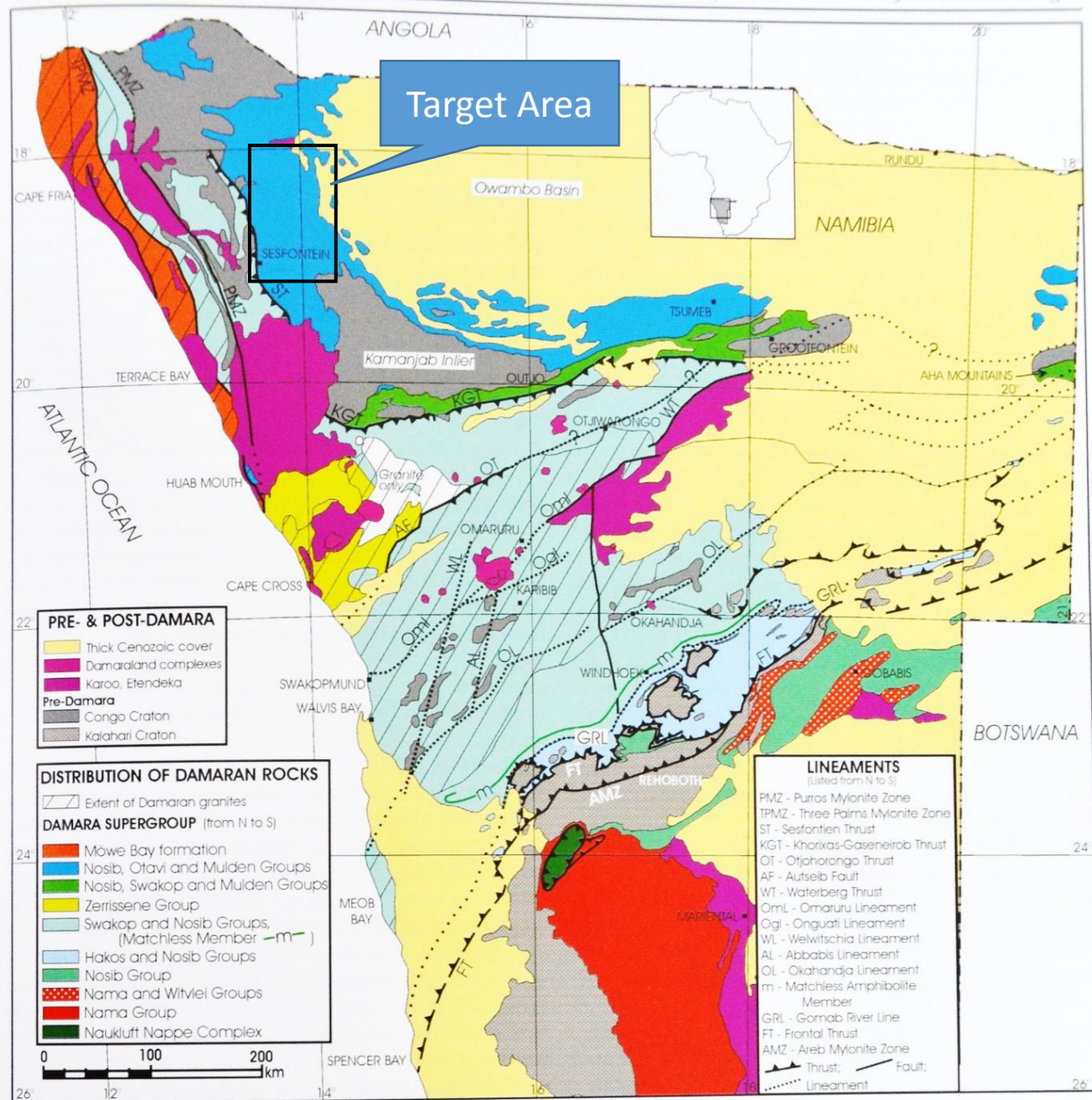
Figure 13.3. Distribution of the main stratigraphic units of the Damara Supergroup.
