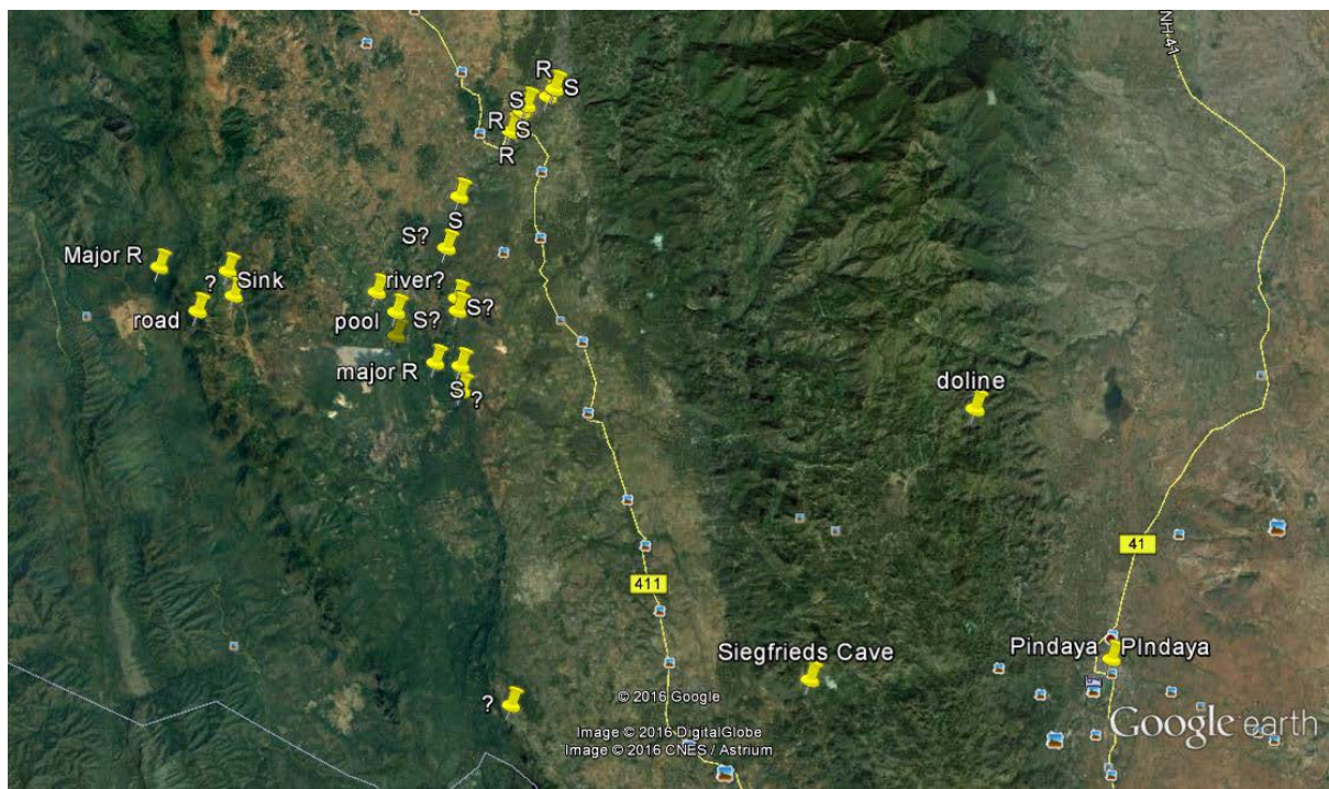
Figure 3. Plateau and escarpment to northwest of Siegfried's Cave.
