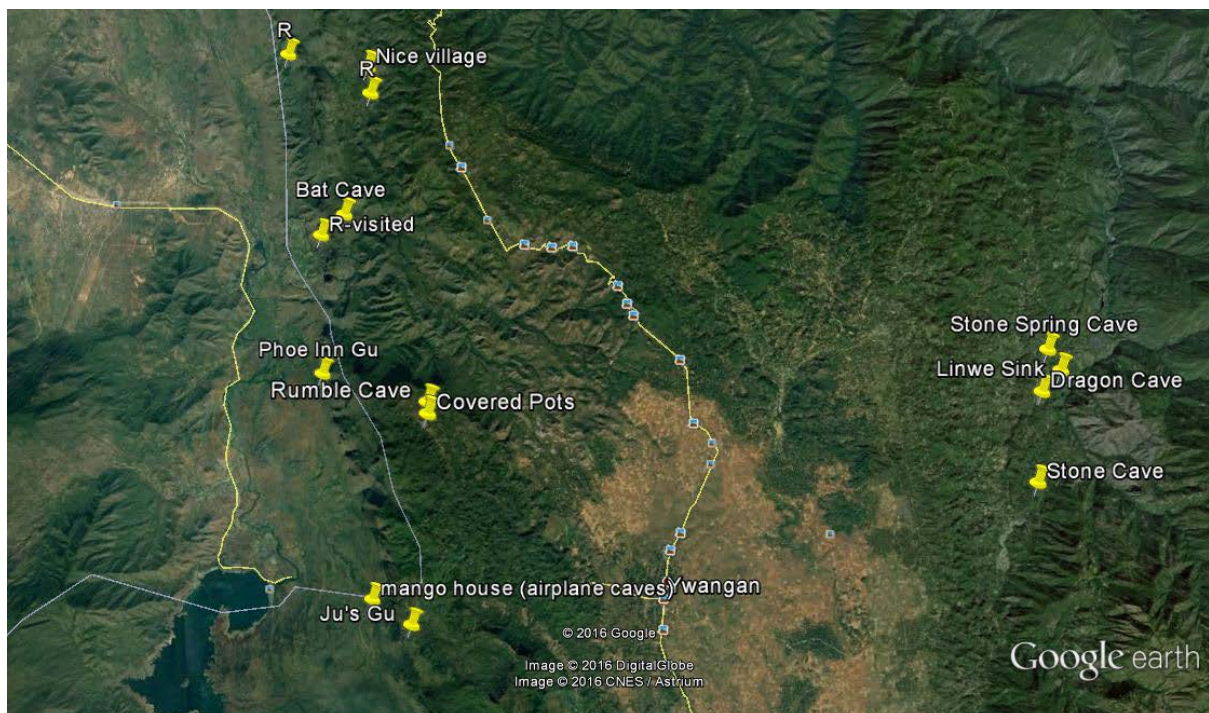
Figure 4. Ju's Gu and the area to the west of Ywangan. It also shows Stone Cave and Dragon Cave etc, which we found in 2012 and is the longest cave currently in Myanmar.
